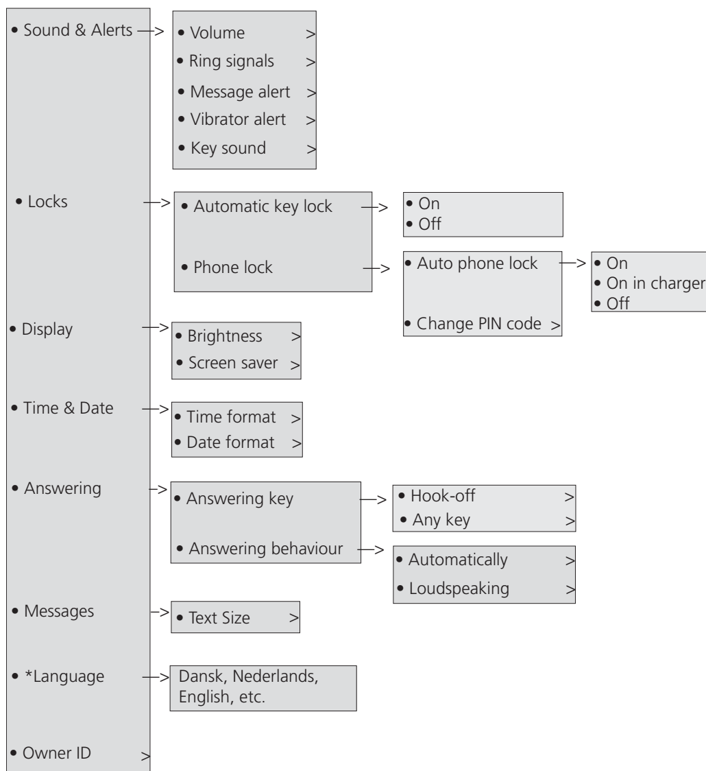
Figure 11 Settings structure
