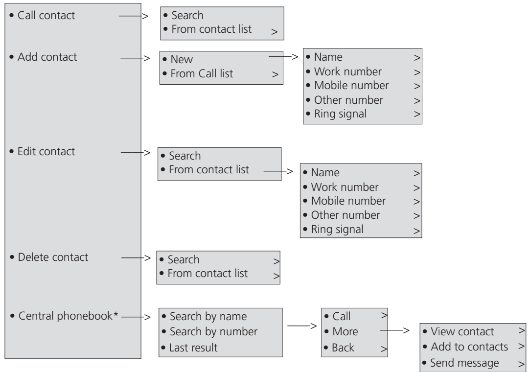
Figure 6 Contacts structure
