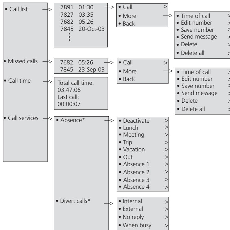
Figure 5 Calls structure
